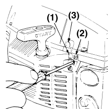
(1) L needle (2) H needle (3) Idle adjusting screw
