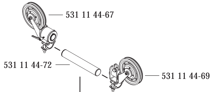
Offset pulley system 504 01 21-01
