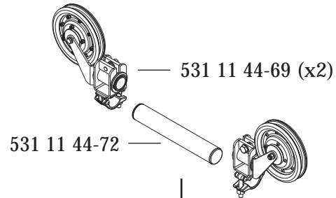
Offset pulley system 504 01 19-01
